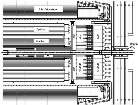
FIGURE 4.7: Side view of the backward region of the H1 detector. The positions of the electromagnetic and hadronic sections of the SPACAL calorimeter and of the BDC are shown.
