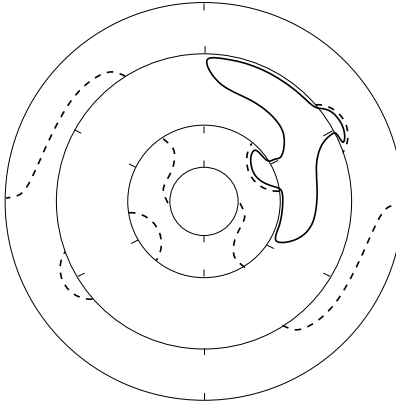
FIGURE 5. The dividing set on \hat{S} for the configuration in the case (b).
