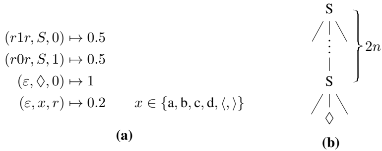
Figure 3.5: (a) WTA M from Ex. 3.3.1. (b) Shape of trees with nonzero weight in [[M]] , where n \in \mathbb{N} .
