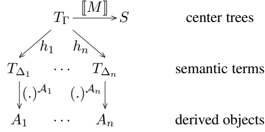
Figure 4.1: Overview of the concept IRTG.
