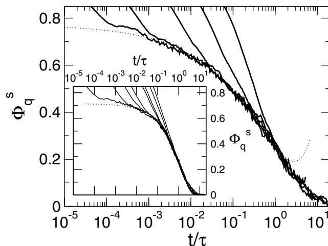
FIG. 3. Correlation functions vs rescaled time t/\tau for \phi_c = 0.4 and \phi_p = 0.375, 0.39, 0.40, 0.415 , and 0.425 (from right to left), and the von Schweidler fit. Inset: same plot for soft spheres and \phi_c = 0.53, 0.54, 0.55, 0.56, 0.57, 0.58, 0.585 , and 0.59 , and the MCT master curve [22].
