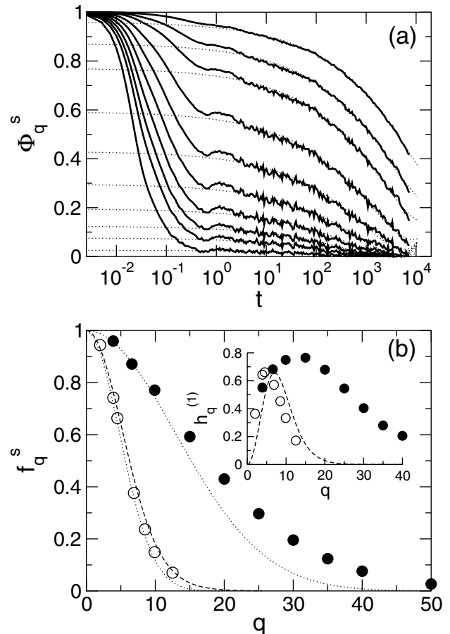
FIG. 2. (a) Correlation functions at \phi_c = 0.4 , \phi_p = 0.425 and von Schweidler fits. From top to bottom, q = 3.9, 6.9, 9.9, 15, 20, 25, 30, 35, 40 , and 50 . (b) f_q^s for glass ( \circ ) and gel ( \bullet ) [from (a)] transitions, with the Gaussian approximation for both of them (dotted lines) and the MCT result for hard spheres (dashed line) [22]. Inset: h_q^{(1)} using \tau from Fig. 1 and the MCT result for hard spheres.
