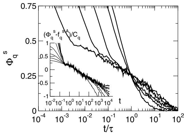
FIG. 5. Correlation function vs rescaled time, t/\tau , at q = 20 . \phi_c = 0.55 , and \phi_p = 0.325, 0.34, 0.35, 0.365 , and 0.375 from right to left at t < \tau . Inset: (\Phi_q^s(t) - f_q)/C_q as a function of time for the same state and wave vectors as Fig. 4 (wave vectors increasing from top to bottom).
