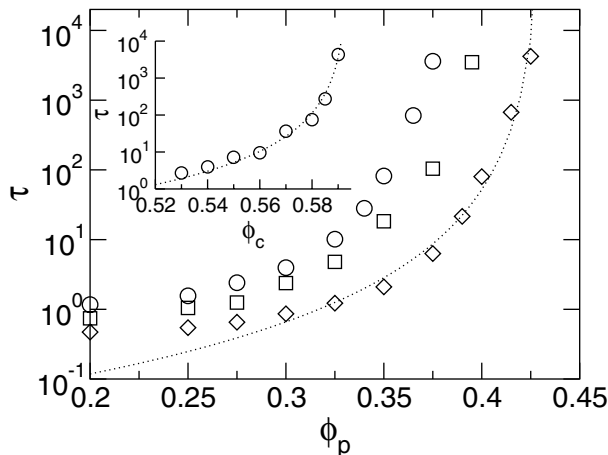
FIG. 1. Relaxation time \tau as a function of \phi_p for three colloid volume fractions: \phi_c = 0.40 ( \diamond ), \phi_c = 0.50 ( \square ), \phi_c = 0.55 ( \circ ). Inset: \tau vs \phi_c for soft spheres [ \phi_p = 0 , V(r) \sim r^{-36} ]. The dotted lines are fittings with predetermined \gamma .
