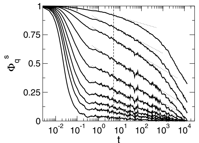
FIG. 4. Same as Fig. 2(a) for \phi_c = 0.55 and \phi_p = 0.375 . Dotted lines: logarithmic fittings to the correlators around f_q . The dashed line represents t_1 .
