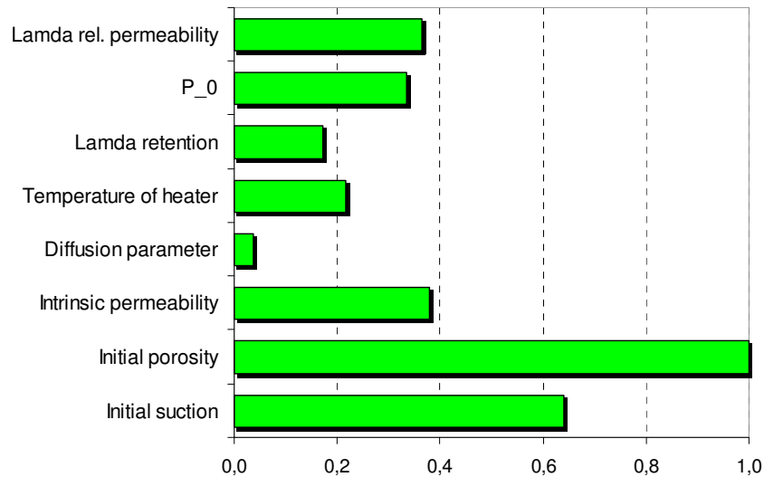
Fig. 6.2: \gamma values for the evolution of degree of saturation with respect to the parameters in group 1
