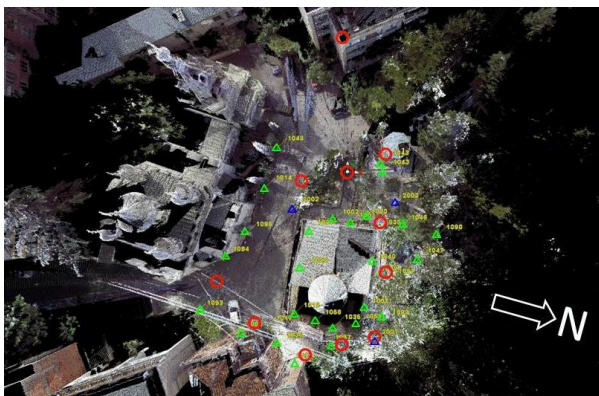
Figure 4. Overview of the registered Faro total point cloud with distribution of positions (red) and target marks (paper marks green, profit targets blue)
