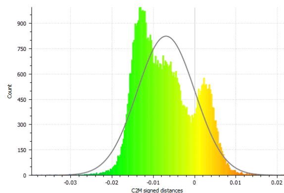
Figure 14. Comparison of the point cloud calculated with RealityCapture (BLK360 and images) compared to Faro
