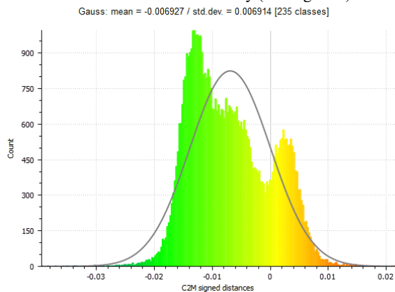
Figure 14c and d show the corresponding histograms of the deviations in the lower and upper areas of the façade. Here it becomes visible that in the upper range worse data are available, analogous to the result from section 2.4.2.
