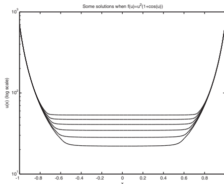
Figure 5: Some solutions when f(u) = u^2(1 + \cos u)
