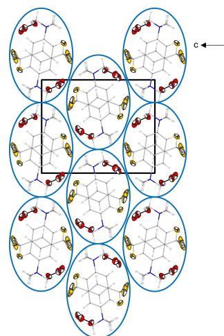
Figure 2. Projection of the crystal structure of [\text{NMe}_3(\text{C}_6\text{H}_4(\text{CF}_3))]\text{O}_3 along [100] . Except fluorine and oxygen, all atoms are represented as wire and stick representation. Thermal ellipsoids for all other atoms are set at 70% probability level. Hydrogen in white, nitrogen in blue, carbon in grey, fluorine in yellow and oxygen in red colour. Rotational \text{CF}_3 disorder and (\text{O}_3)^- disorder is omitted for clarity.
