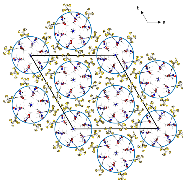
Figure 1. Projection of the crystal structure of [\text{NMe}_3(\text{C}_6\text{H}_3(\text{CF}_3)_2)][\text{ONOO}] \cdot 1/3 \text{NH}_3 along [001] . Margins of the unit cell are shown in black, blue circles highlight the hexagonal dense rod packing. Fluorine, peroxyxynitrite and ammonia are presented as thermal ellipsoids set at 70% probability level, all other atoms are drawn in wire and stick representation. Hydrogen in white, nitrogen in blue, carbon in grey, fluorine in yellow and oxygen in red colour.
