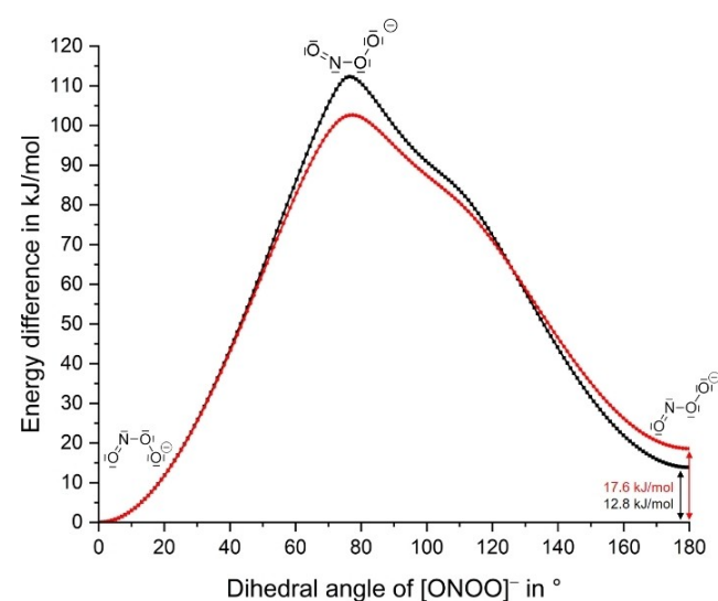
Figure 7. Relaxed dihedral surface scan ( 0-180^\circ in 1^\circ steps) with solvent module CPCMC( \text{NH}_3 ) (red) and level without (black) at B3LYP-D3(BJ)/aug-cc-pVTZ level of theory (Orca 5.0.3).
