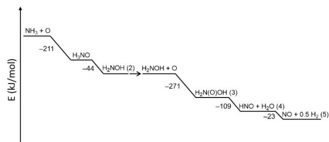
Scheme 3. Reaction scheme for the in-situ formation of NO from ammonia and mono-oxygen at B3LYP-D3(BJ)/aug-cc-pVTZ CPCMC(NH 3 ) level of theory (Orca 5.0.3).
