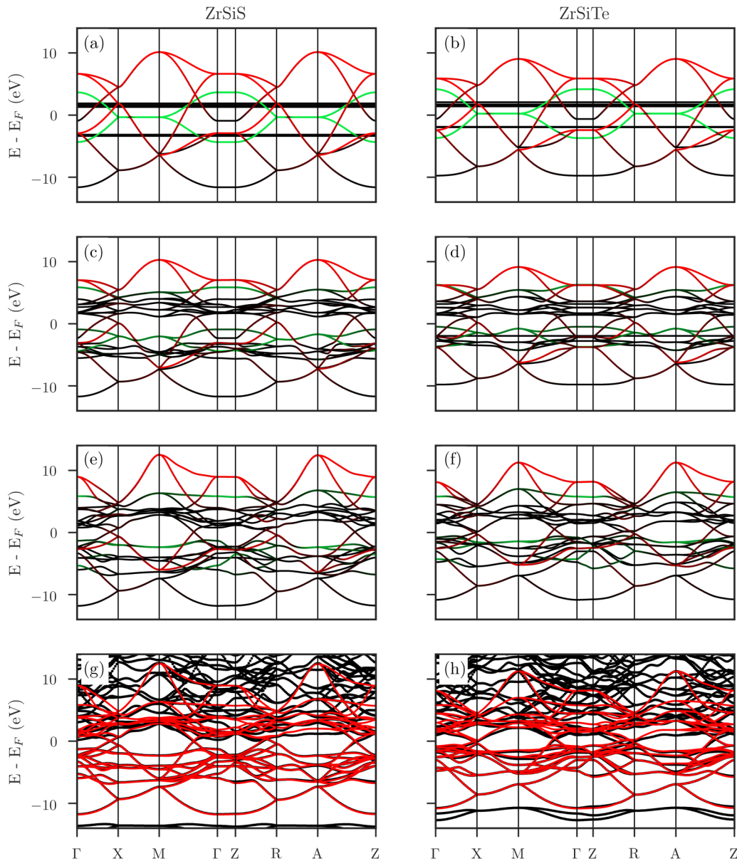
FIG. 5. Wannier band structures of ZrSiS (left) and ZrSiTe (right). The red and green colors in panels (a)–(f) reflect the Si pxpy and Si pz weights, respectively. Panels (a)–(f) show the band structures obtained for hopping constrained to: nearest neighbors on the Si plane (a) and (b), nearest-neighbors Si-Si, Si-Zr, and Zr-S/Te (c) and (d), and no constraints (e) and (f). Panels (g) and (h) show the same Wannier band structure (red) as panels (e) and (f) compared to the full DFT band structures (black).
