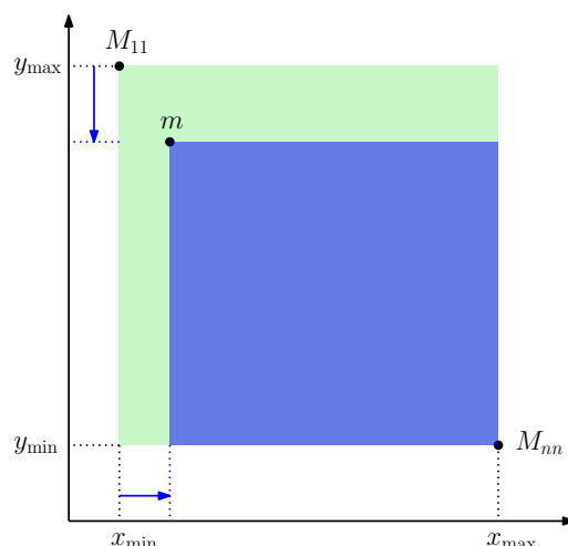
■ Figure 4 Initial search range (green rectangle) spanned by M_{11} and M_{nn} . The range-minimum element m then leads to a reduction of y_{\max} and an increase of x_{\min} (blue arrows) which tightens the search range for the next element of C .
