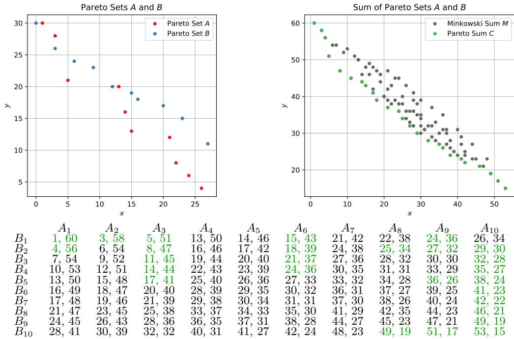
■ Figure 1 Example instance with input Pareto sets A, B of size 10. The Minkowski sum has 100 elements. The Pareto sum C consists of 27 elements (marked green in the plot as well as in the matrix representation).
