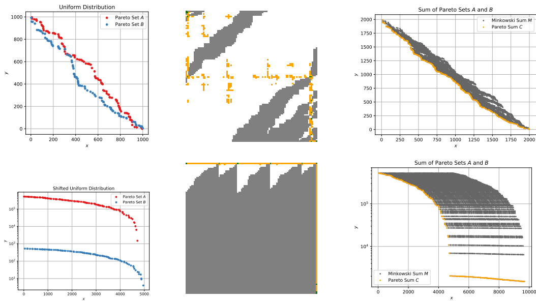
■ Figure 5 Example instances for uniform and shifted uniform point distributions. For the latter, note the logscale of the y-axis. The color coding is the same as in Figure 3.
