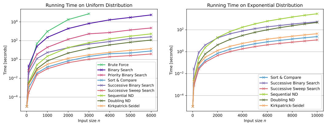
■ Figure 6 Average running times of all algorithms on uniform distributions (left) and of the top six algorithms on exponential distributions (right). Note the logscale of the y-axis.
