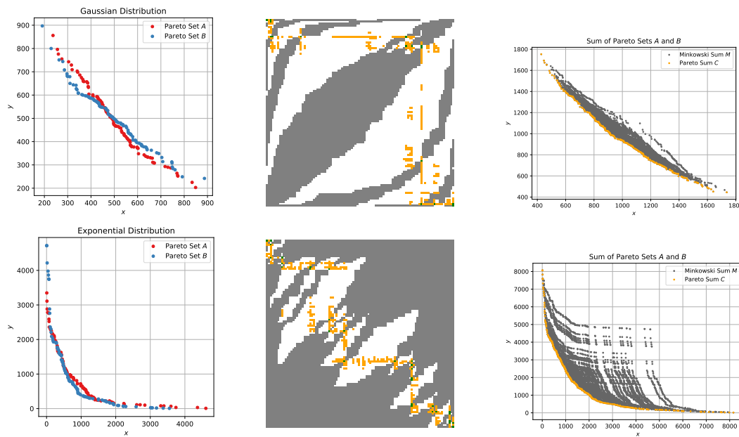
■ Figure 3 Input Pareto sets following different kinds of distributions (left) and schematic depiction of the corresponding Minkowski matrix M (middle). Green dots indicate entries in M that are points on the Minkowski sum of the convex hulls of A and B , black dots indicate entries that are dominated by the green ones, and orange dots encode the remaining elements of the Pareto sum which then together dominate the white dots. In the right images, the Minkowski sum and the Pareto sum are illustrated based on point coordinates.
