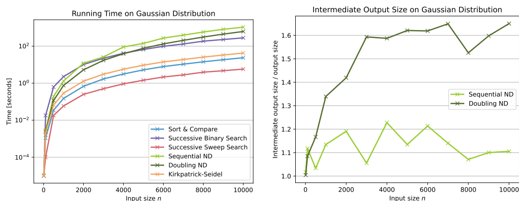
■ Figure 7 Left: Average running times of selected algorithms on Gaussian distribution. Right: Intermediate output size of the Sequential ND and Doubling ND algorithms.
