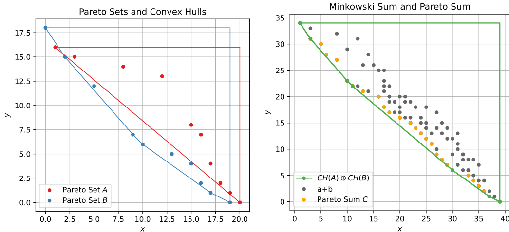
■ Figure 2 Left: Pareto sets A, B together with their convex hulls. Right: The Minkowski sum CH(A) \oplus CH(B) of the convex hulls encloses all pairwise vector additions a + b with a \in CH(A) and b \in CH(B) . The respective vertices (green points) are a subset of the Pareto Sum C .
