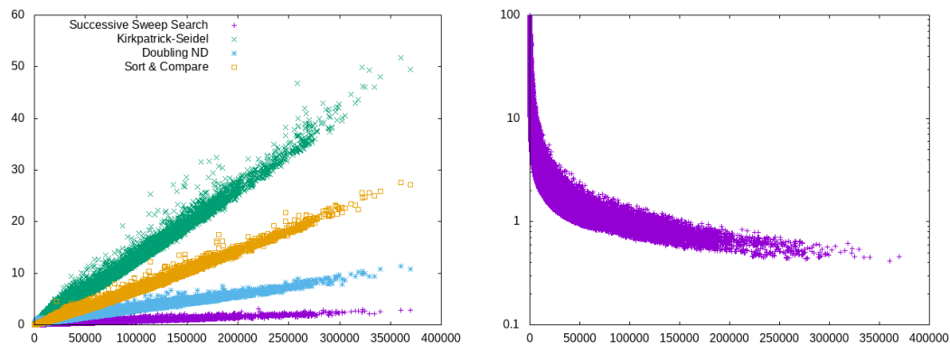
■ Figure 8 Detailed results for the ROAD2 instance. Left: Running times in seconds per Pareto sum computation in dependency of the size of the Minkowski sum. Right: Pareto sum size as percentage (logscale) of the size of the Minkowski sum.
