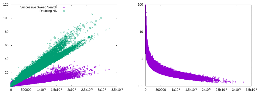
■ Figure 9 Detailed results for the ROAD3 instance. Left: Running times in seconds per Pareto sum computation in dependency of the size of the Minkowski sum. Right: Pareto sum size as percentage (logscale) of the size of the Minkowski sum.
